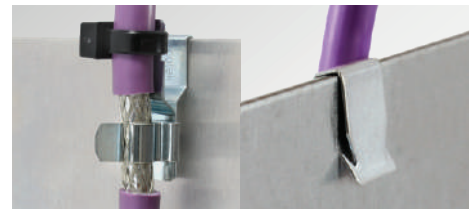
EMC shield clamps for assembly on sheet edges with/without strain relief function, single and double
