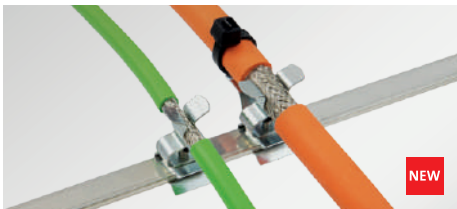
EMC shield clamps for 10 × 3 mm bus bars with/without strain relief function, single and double
