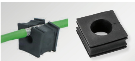
Split EMC grommets for cables with and without connectors for cable diameters 2 to 33 mm
