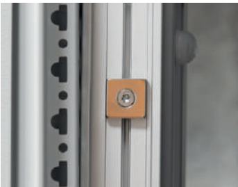
Assembly aid via integrated magnets
