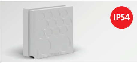
Membrane cable grommets IP54 protection, high cable density for cable diameters 6.5 to 14.5 mm QT-DT 122
