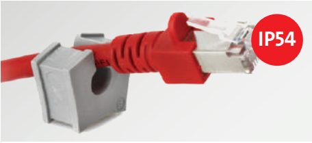
Split cable grommets, single IP54 protection for cable diameters 1 to 15 mm QT 120
