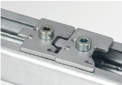
SC single for C-rail with twist protection notch (36231)
