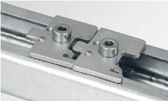
SC mounting foot for C-rail with twist protection notch
